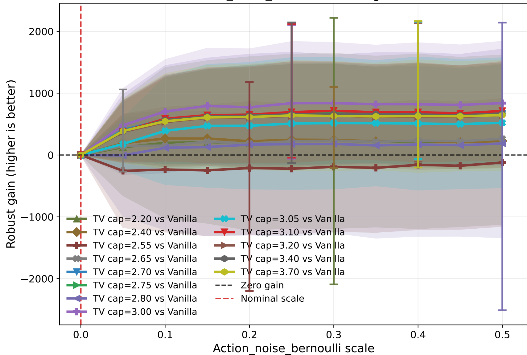
Action_noise_bernoulli robust gain
